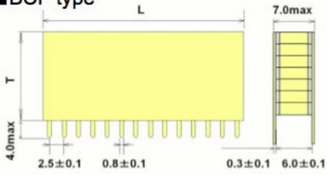
BCF,BSF Dimensions (Capacitance)
