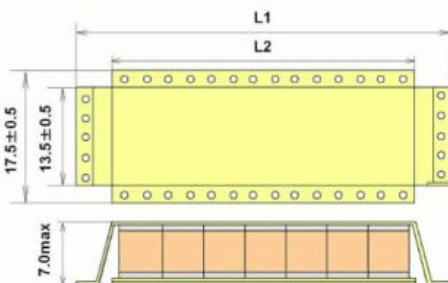
BCS Dimensions (Capacitance)
