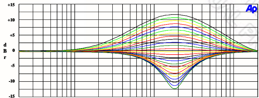
Figure 16: EQ Band 4 Peak Filter Gains for Lowest Cut-Off Frequencies with EQ4BW = 0
