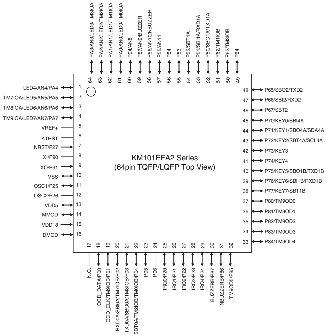
Figure:1.3.4 Pin Configuration (KM101EFA2 Series 64-pin TQFP/LQFP)
