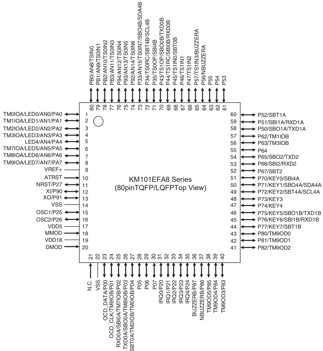
Figure:1.3.1 Pin Configuration (KM101EFA8 Series 80-pin TQFP/LQFP)
