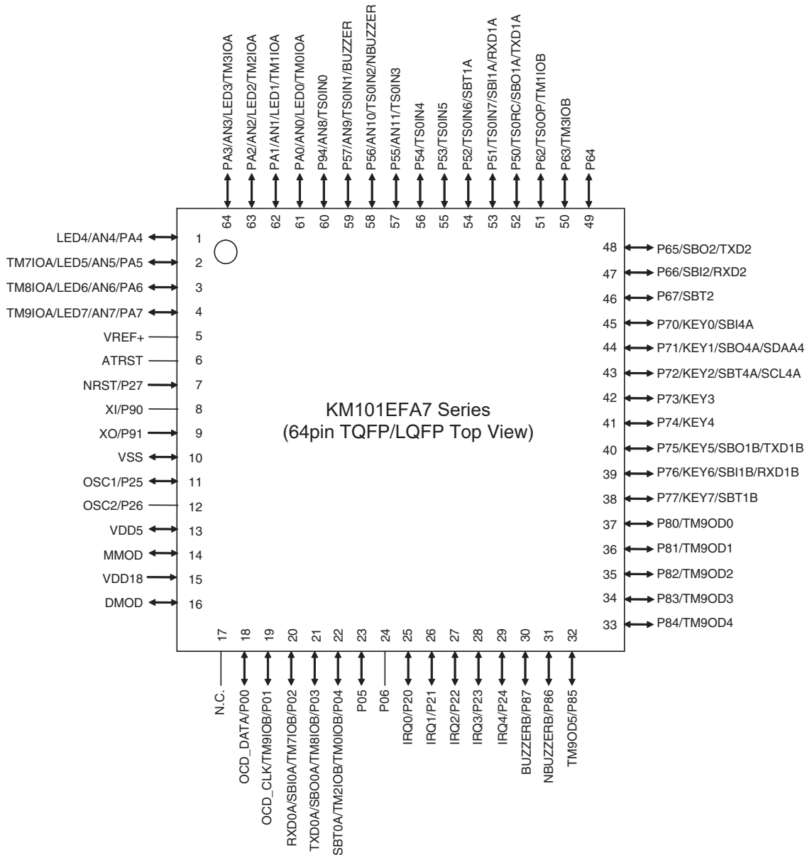
Figure:1.3.2 Pin Configuration (KM101EFA7 Series 64-pin TQFP/LQFP)
