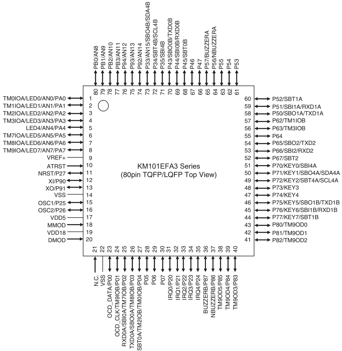
Figure:1.3.3 Pin Configuration (KM101EFA3 Series 80-pin TQFP/LQFP)
