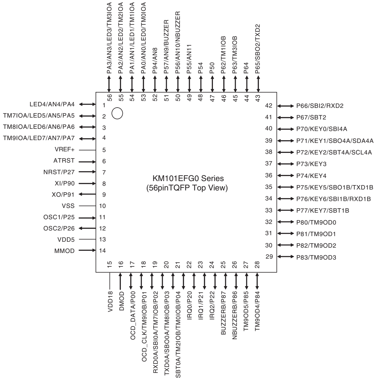
Figure:1.3.5 Pin Configuration (KM101EFG0 Series 56-pin TQFP)
